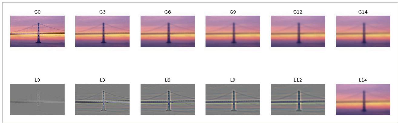
BAY BRIDGE · GAUSSIAN AND LAPLACIAN STACKS
