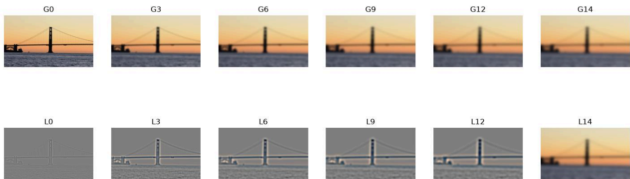
GOLDEN GATE · GAUSSIAN AND LAPLACIAN STACKS
