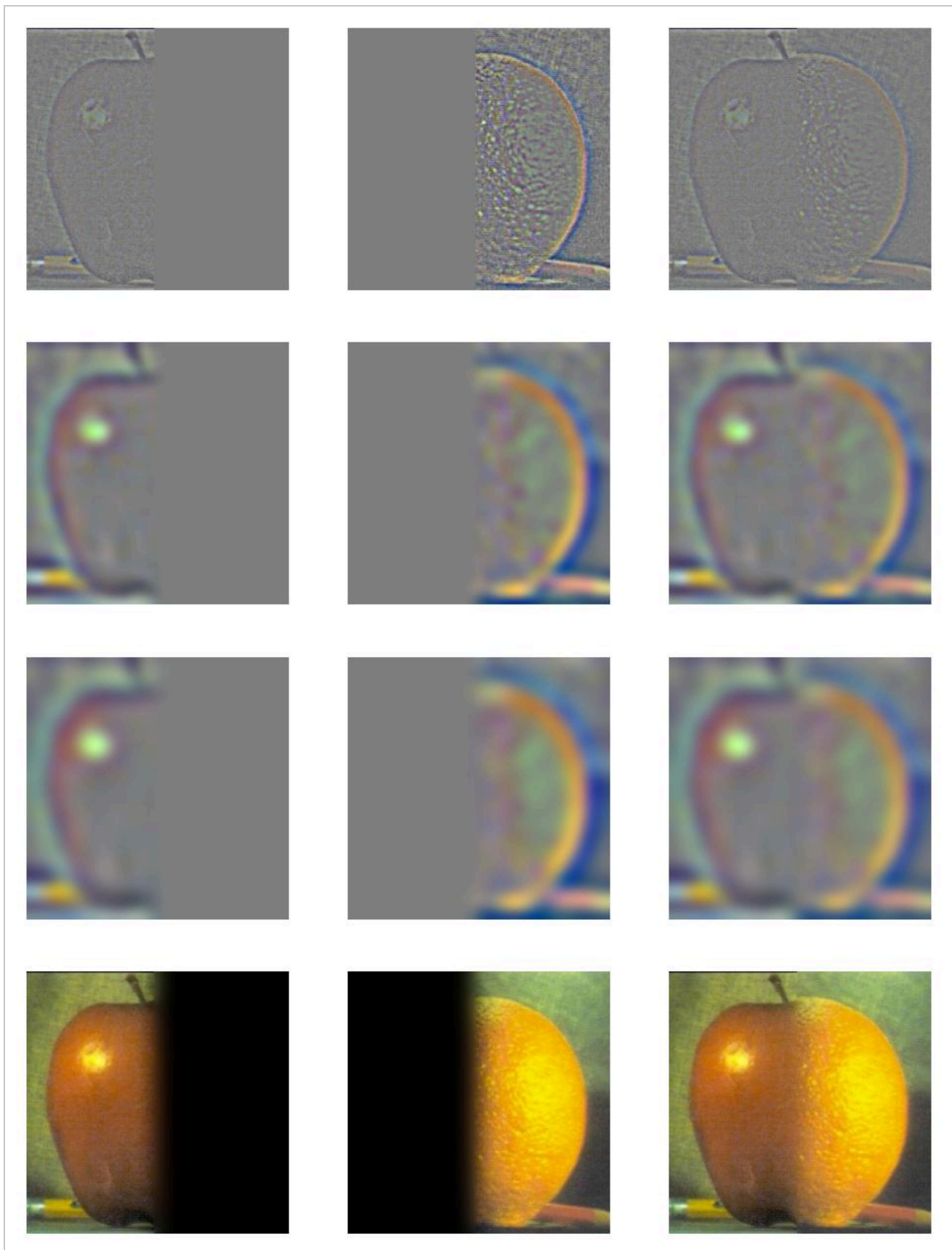
FIGURE 3.42 RECREATION · LEVELS 0, 5, 10, AND THE FULL SUM
